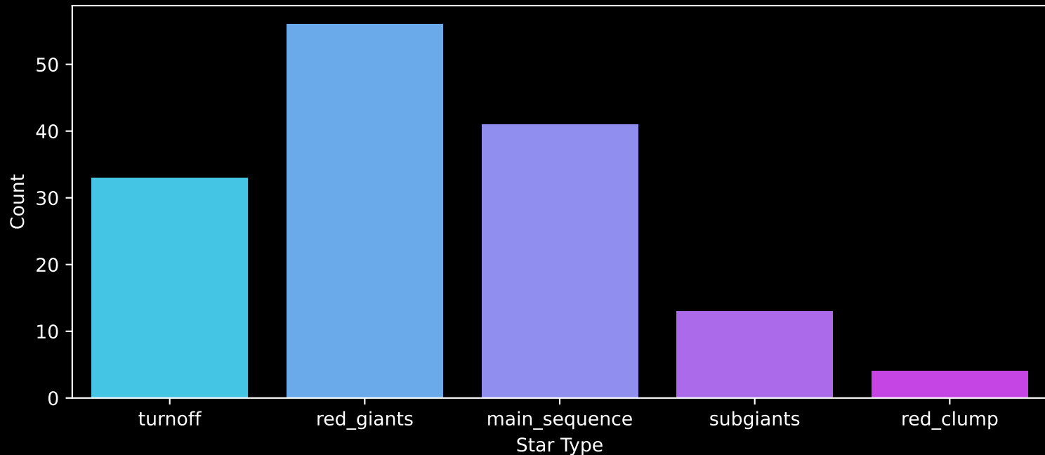
APOGEE DR17 Field: [281-34-O] Count plot of Star Type
