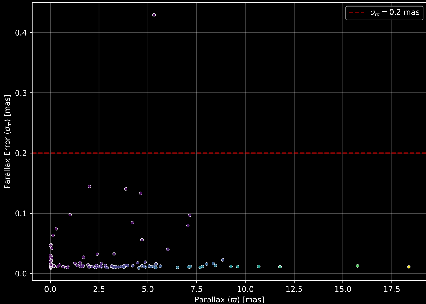
APOGEE DR17 Field: [281-34-O] Parallax Quality (n= 147)
