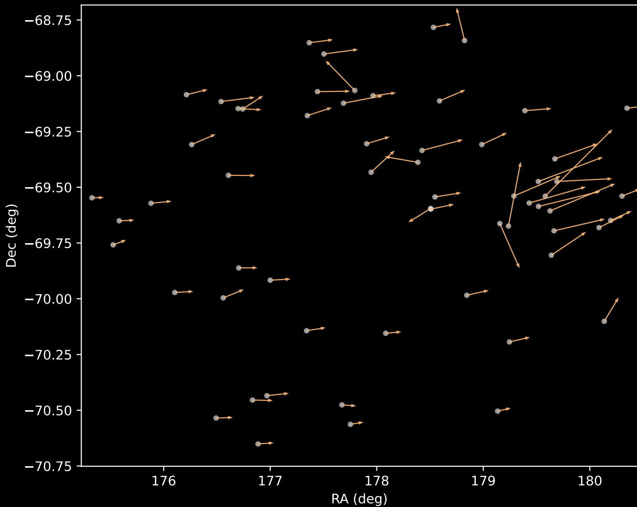
APOGEE DR17 Cluster 3 Proper Motion Vectors (n=61)
