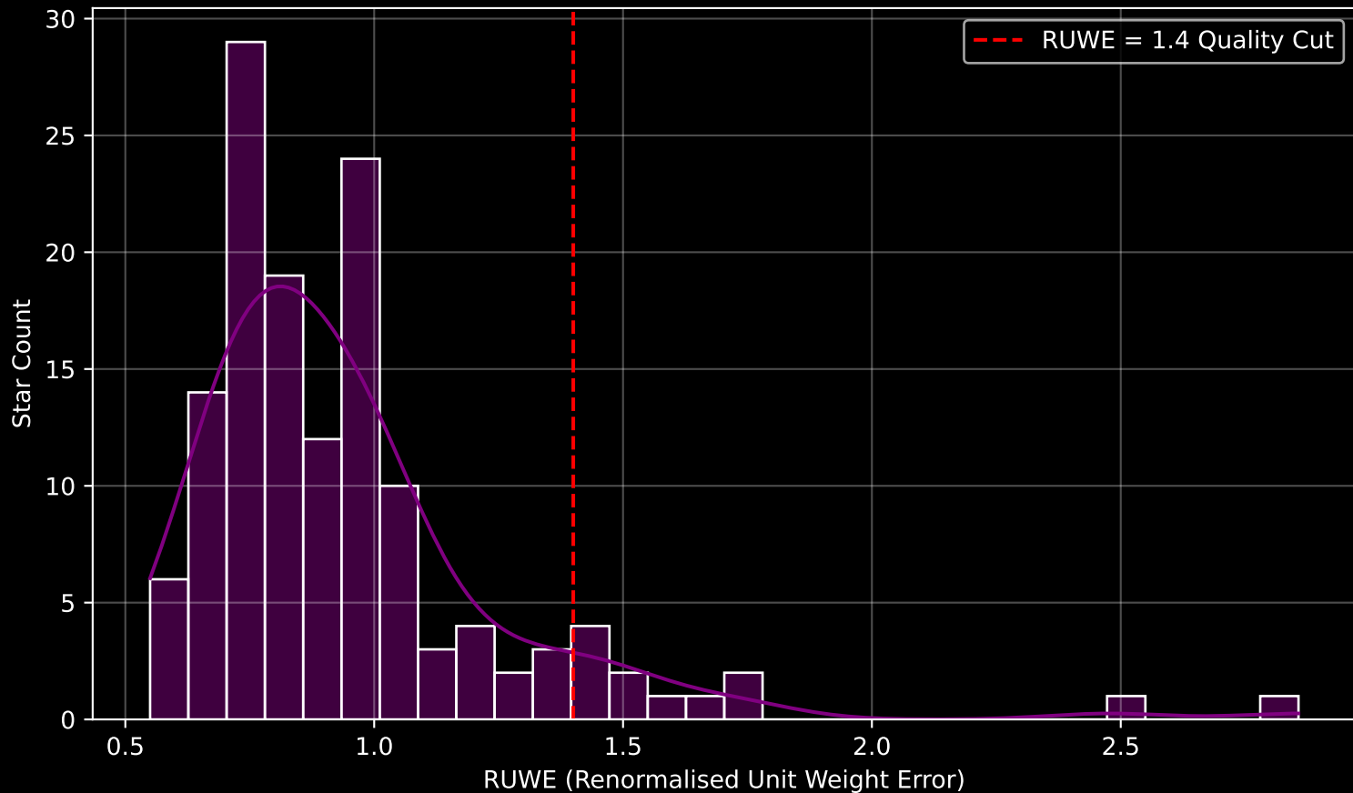
GAPOGEE DR17 Field [281-34-O] RUWE Distribution (n= 138)
